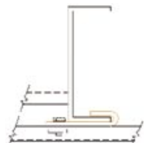
Grapa Guia Ref. CKL 646
